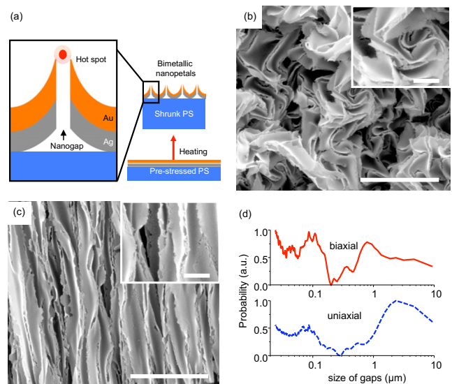
FIG. 1. (Color online) (a) Schematic of fabrication process and creation of hot spots on bimetallic nanopetals. SEM images with large-scale biaxial (b) and uniaxial (c) Au/Ag petals on shrunk PS sheets. The insets in (b) and (c) show corresponding enlarged view of SEM images. The scale bars in (b) and (c) are 10 \mu\text{m} . The scale bars in inset of (b) and (c) are 2 \mu\text{m} . (d) Histograms of gaps dimensions are normalized by their maximum values.
